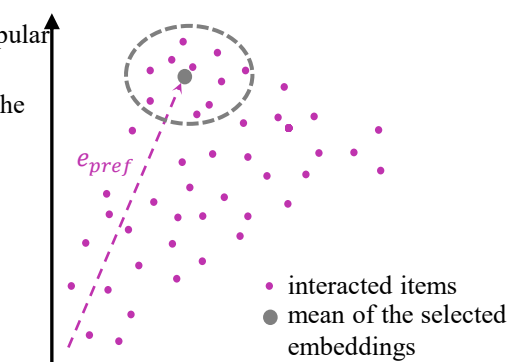
(b) Construction of e_{pref}
