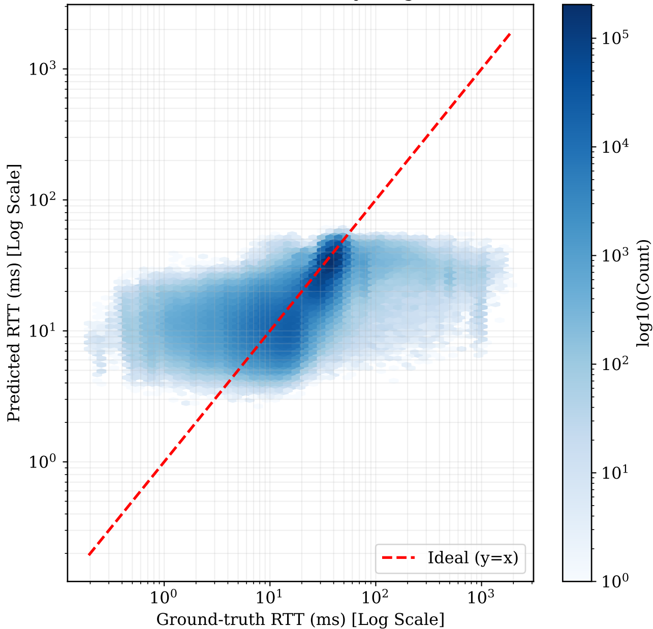
RTT Prediction Accuracy (Log Scale)
