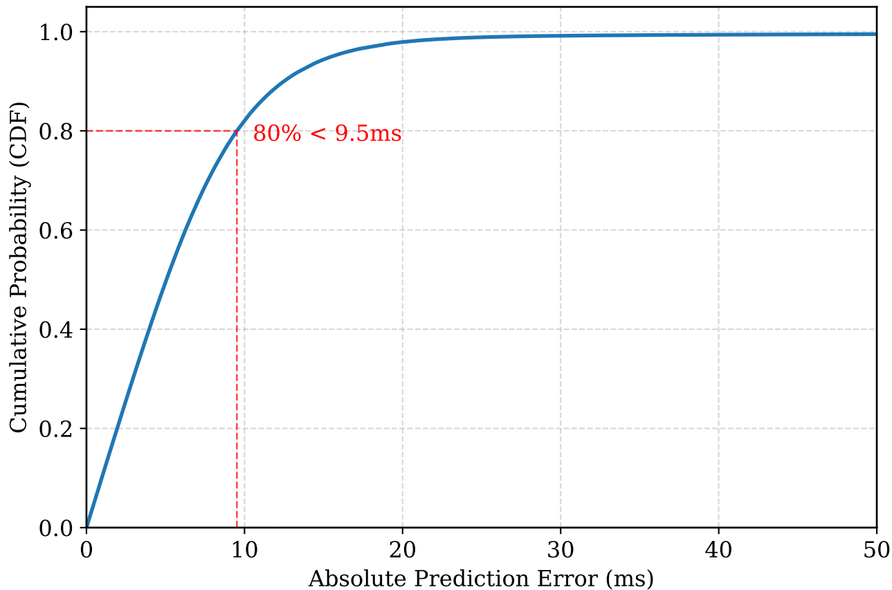
Cumulative Distribution of RTT Prediction Error
