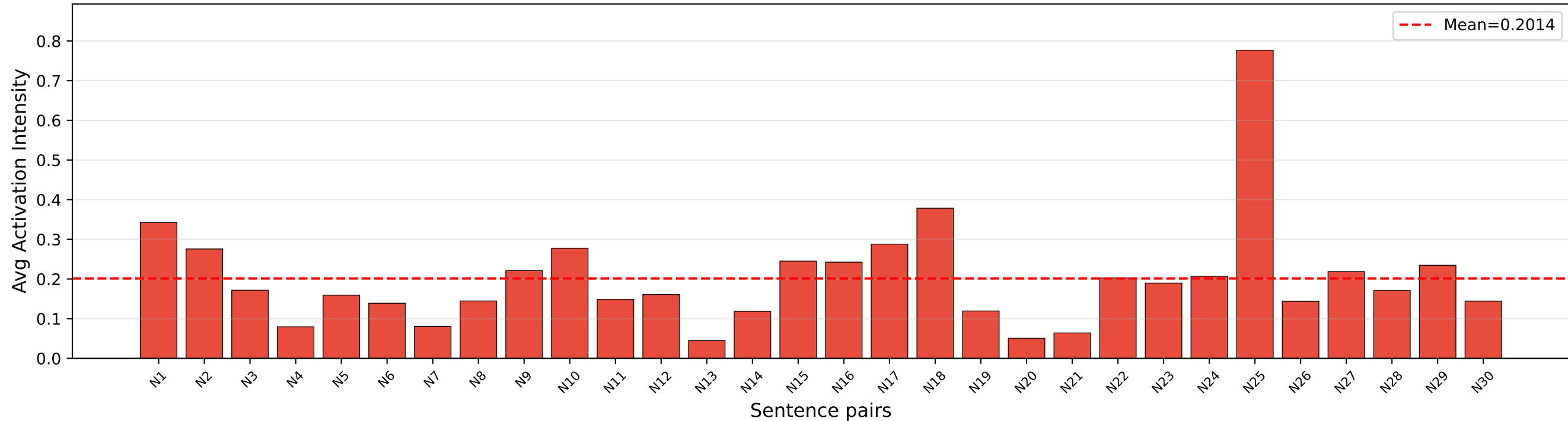
DeepSeek-R1-Distill-Qwen-1.5B (MRPC, L15): Avg Top-5 Non-paraphrase features on Predicted-NO pairs
