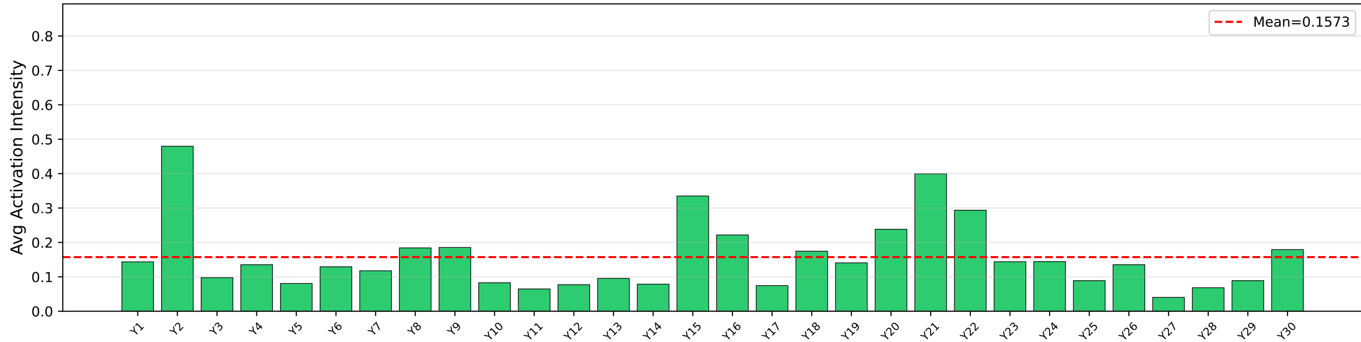
DeepSeek-R1-Distill-Qwen-1.5B (MRPC, L15): Avg Top-5 Non-paraphrase features on Predicted-NO pairs
