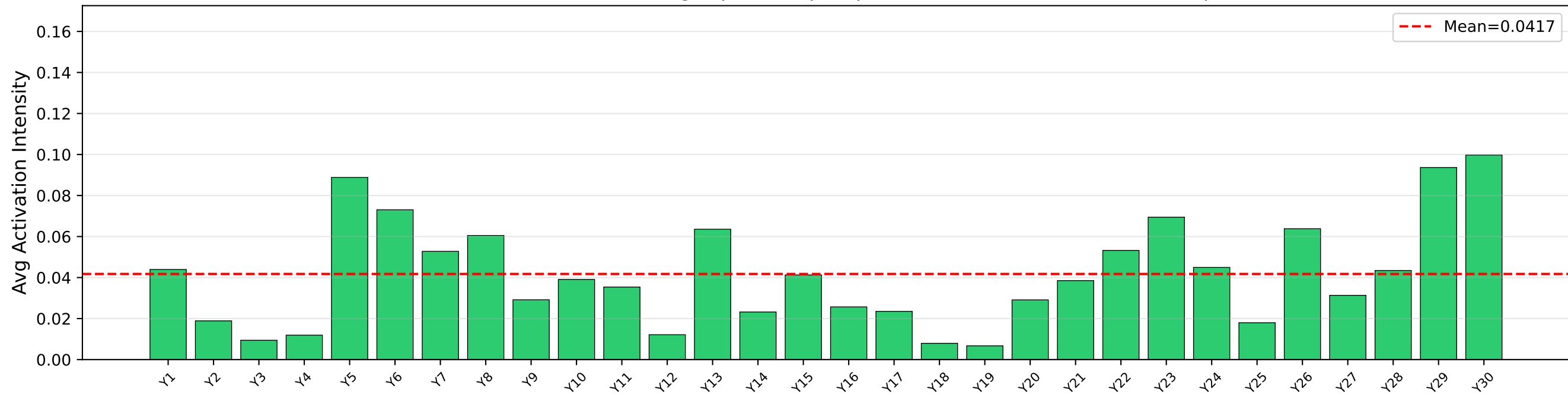
GPT-2 Small (MRPC, L2): Avg Top-5 Non-paraphrase features on Predicted-NO pairs
