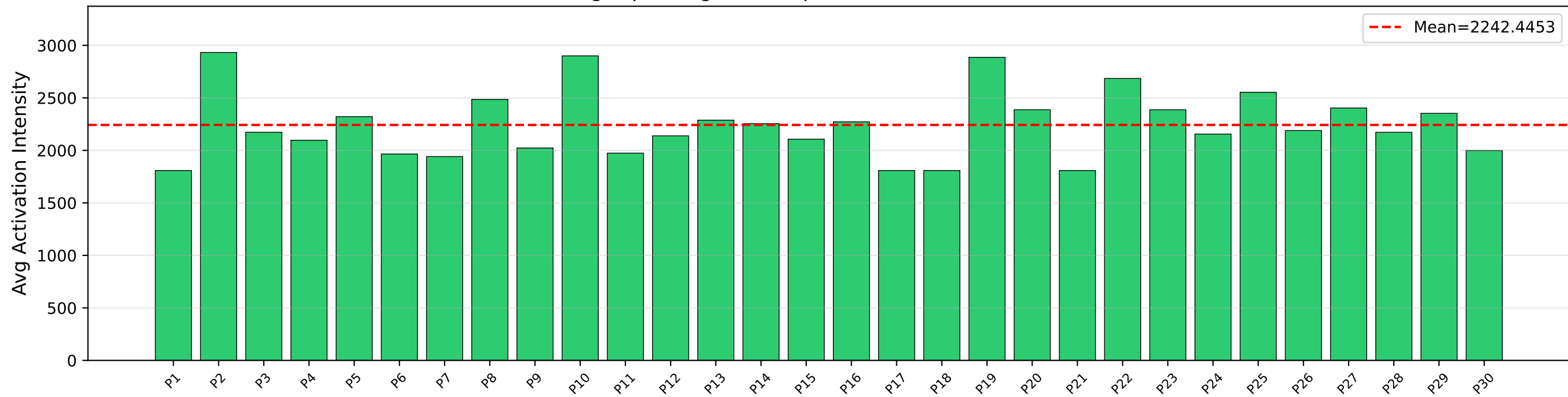
Qwen3-8B: Avg Top-5 Negative-responsible features on Negative Sentences
