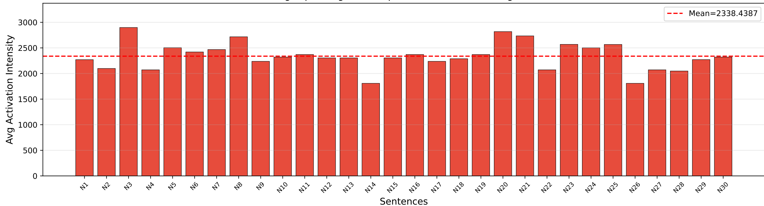
Qwen3-8B: Avg Top-5 Negative-responsible features on Negative Sentences
