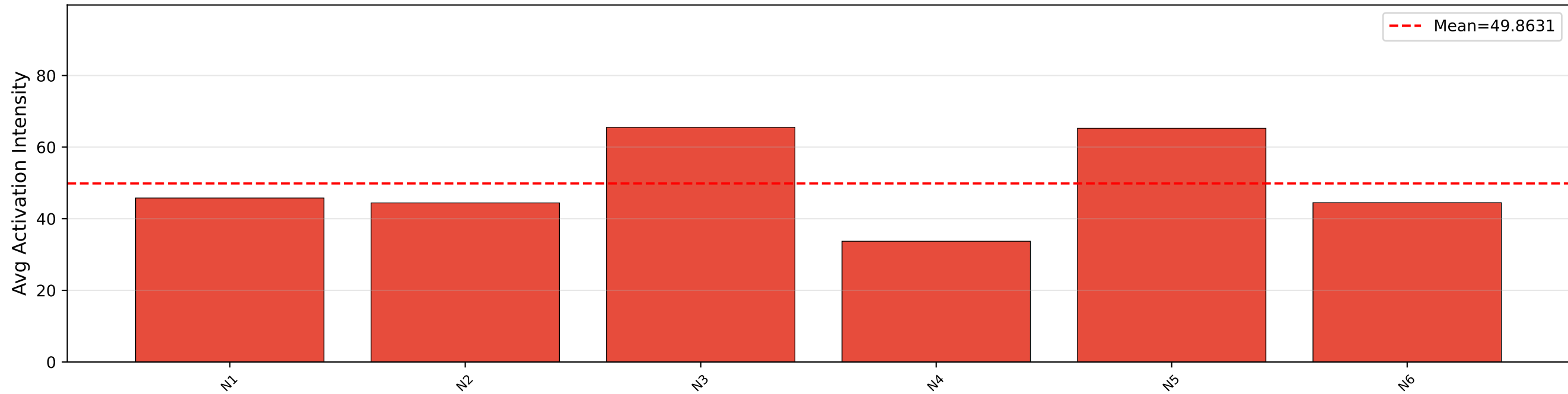
Qwen3-0.6B (MRPC, L14): Avg Top-5 Paraphrase (semantic-sim) features on Predicted-NO pairs
