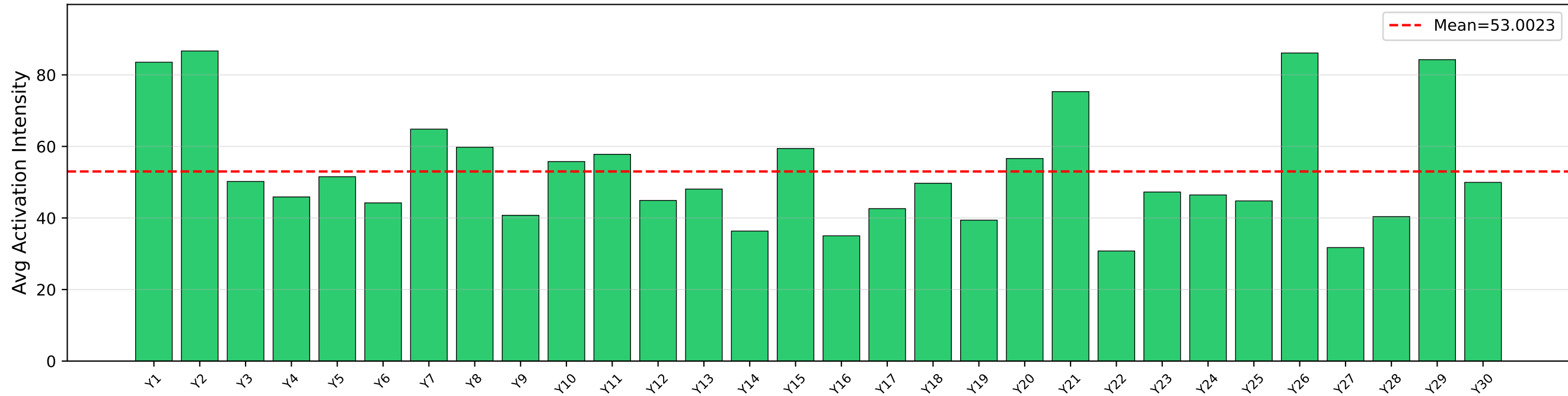
Qwen3-0.6B (MRPC, L14): Avg Top-5 Paraphrase (semantic-sim) features on Predicted-NO pairs
