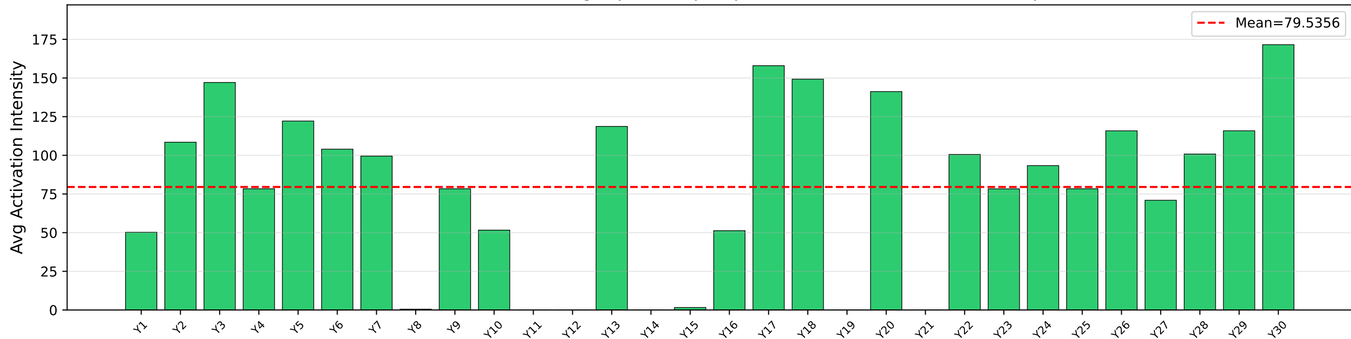
Qwen3-8B (MRPC, L21): Avg Top-5 Non-paraphrase features on Predicted-NO pairs
