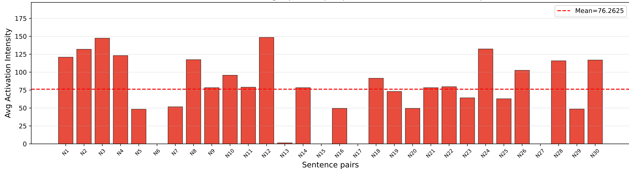
Qwen3-8B (MRPC, L21): Avg Top-5 Non-paraphrase features on Predicted-NO pairs
