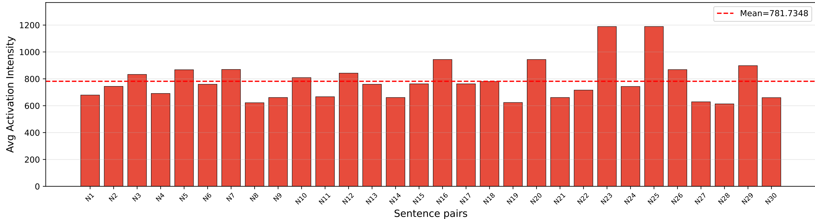
Qwen3-8B (MRPC, L21): Avg Top-5 Paraphrase (semantic-sim) features on Predicted-NO pairs
