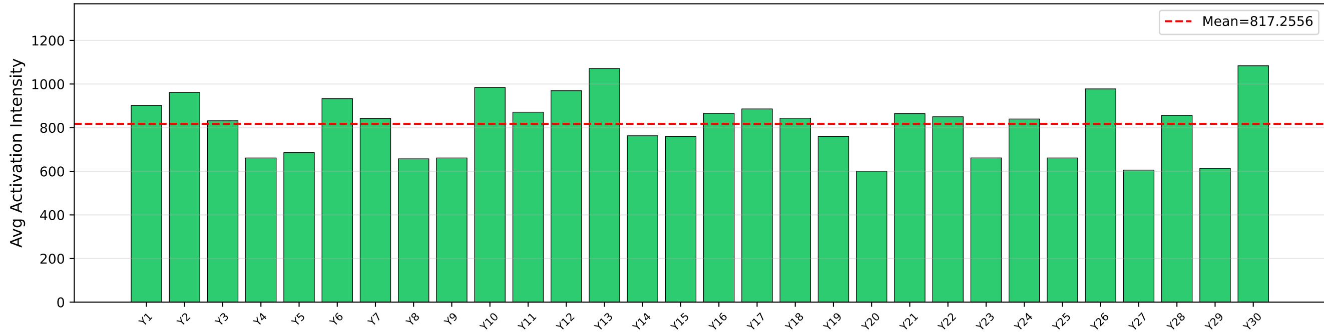
Qwen3-8B (MRPC, L21): Avg Top-5 Paraphrase (semantic-sim) features on Predicted-NO pairs
