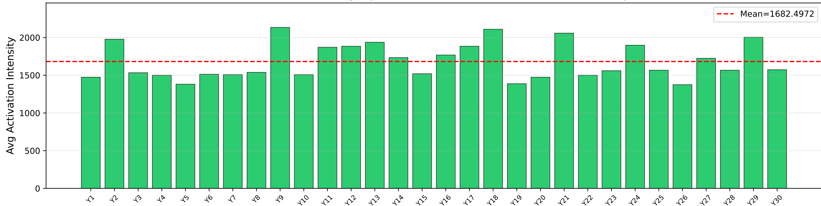
Qwen3-8B (MT, L20): Avg Top-5 Valid-translation features on Predicted-NO pairs
