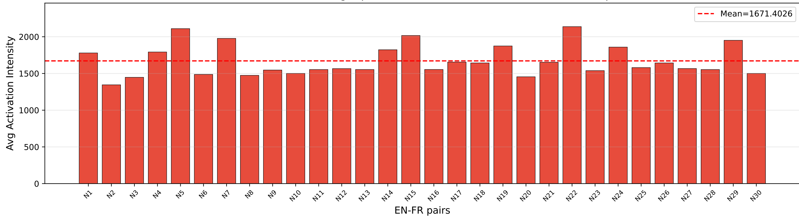
Qwen3-8B (MT, L20): Avg Top-5 Valid-translation features on Predicted-NO pairs
