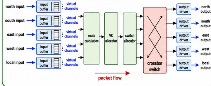
ZOOM: SWITCH NODE
