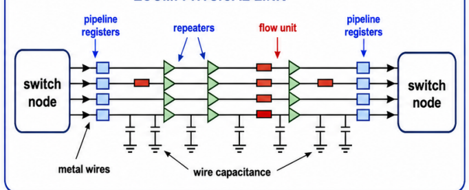
ZOOM: PHYSICAL LINK
