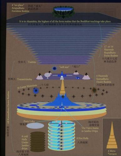
Fig. 3. The Mount Meru world system.
