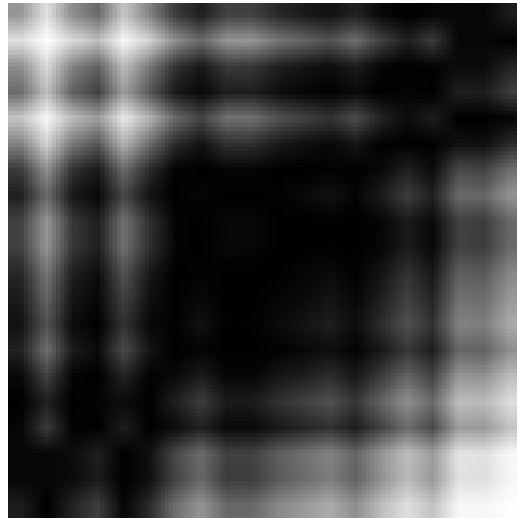
(c) GAF
