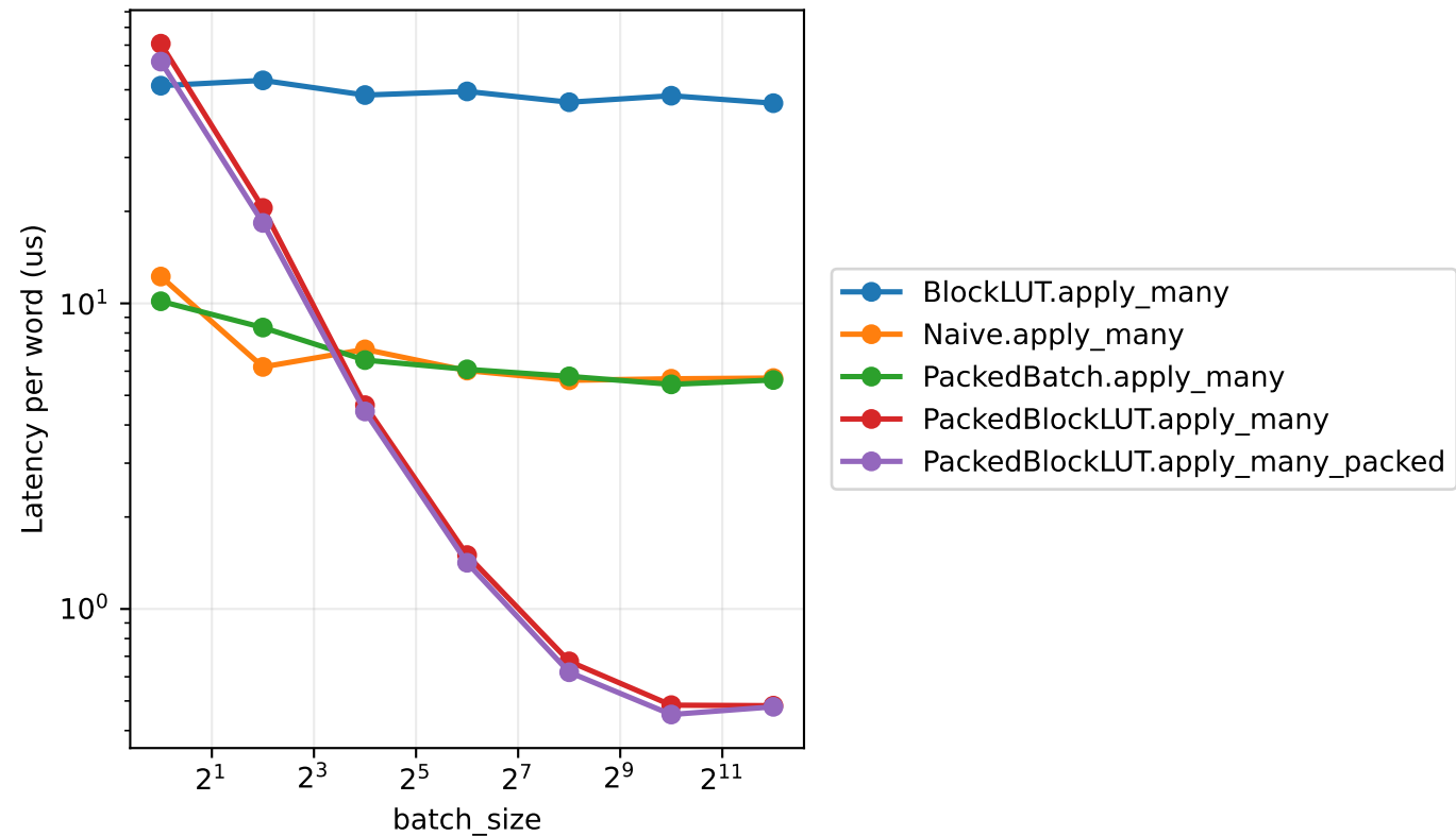
GF(2) batch-size micro-benchmark
