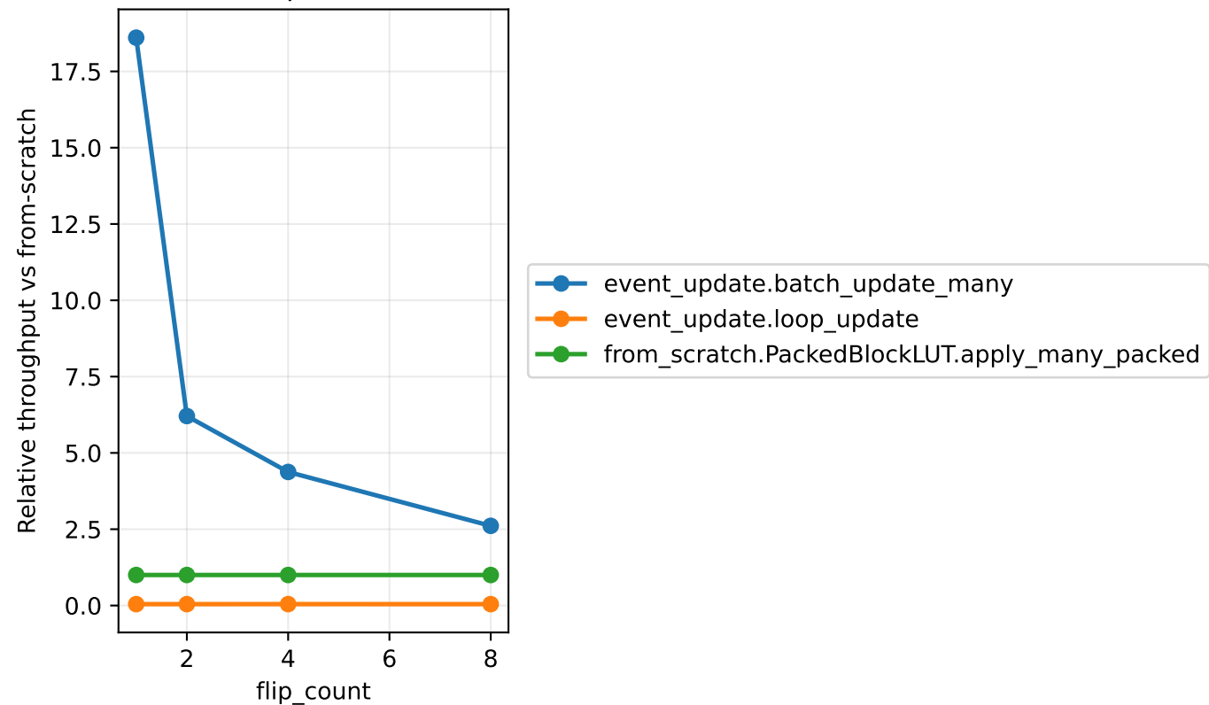
GF(2) event-update benchmark
