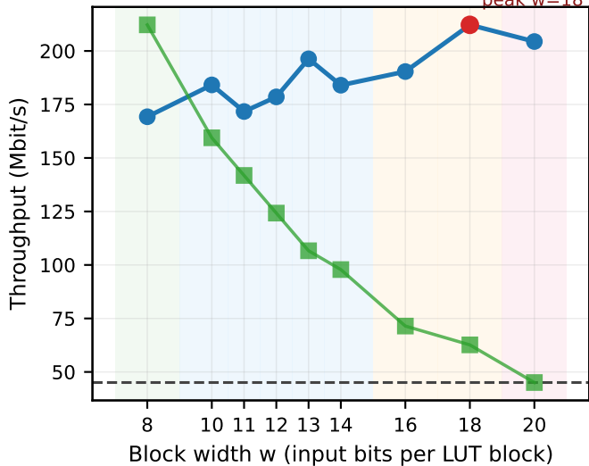
(a) BCH(255,239), r=16 , batch=300000
