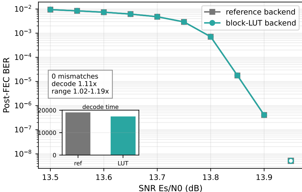
BER overlap with decode-time inset
