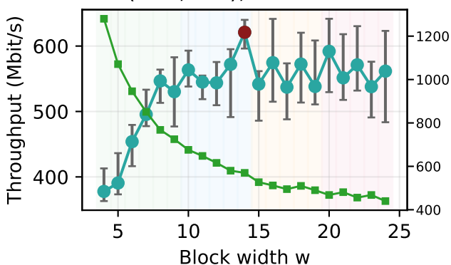
BCH(255,231), r=24: median
