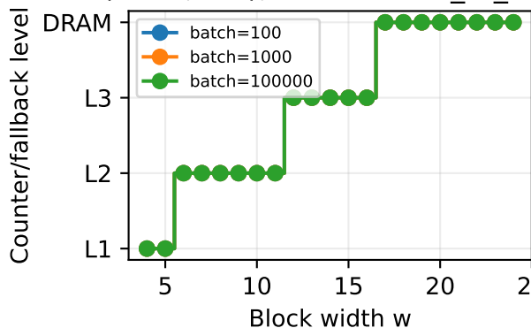
BCH(1023,993), r=30: cache_fit_fallback
