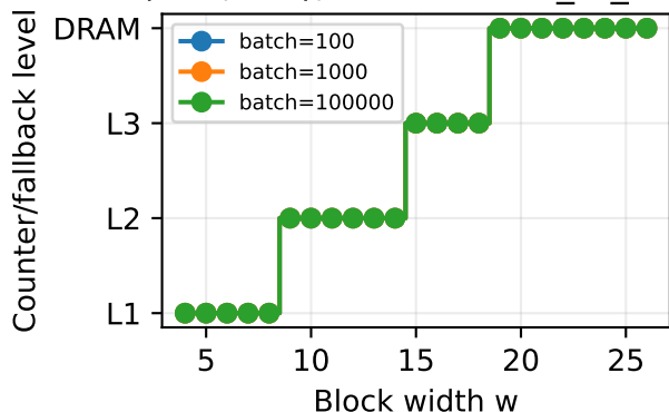
BCH(511,484), r=27: cache_fit_fallback
