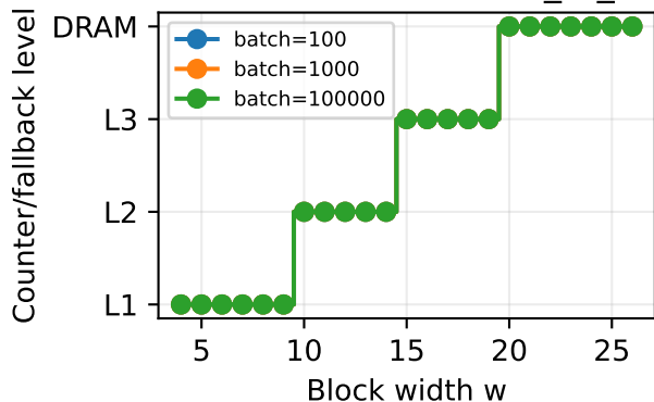
BCH(255,231), r=24: cache_fit_fallback
