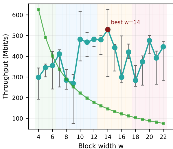
BCH(511,484), r=27, batch=1000
