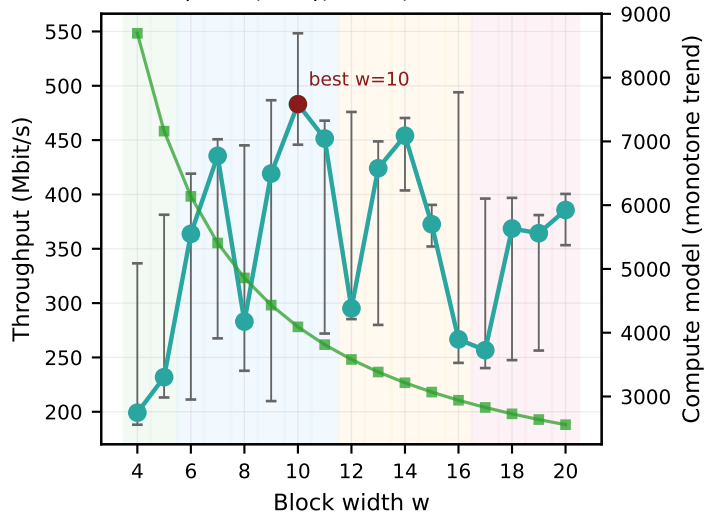
BCH(1023,993), r=30, batch=1000
