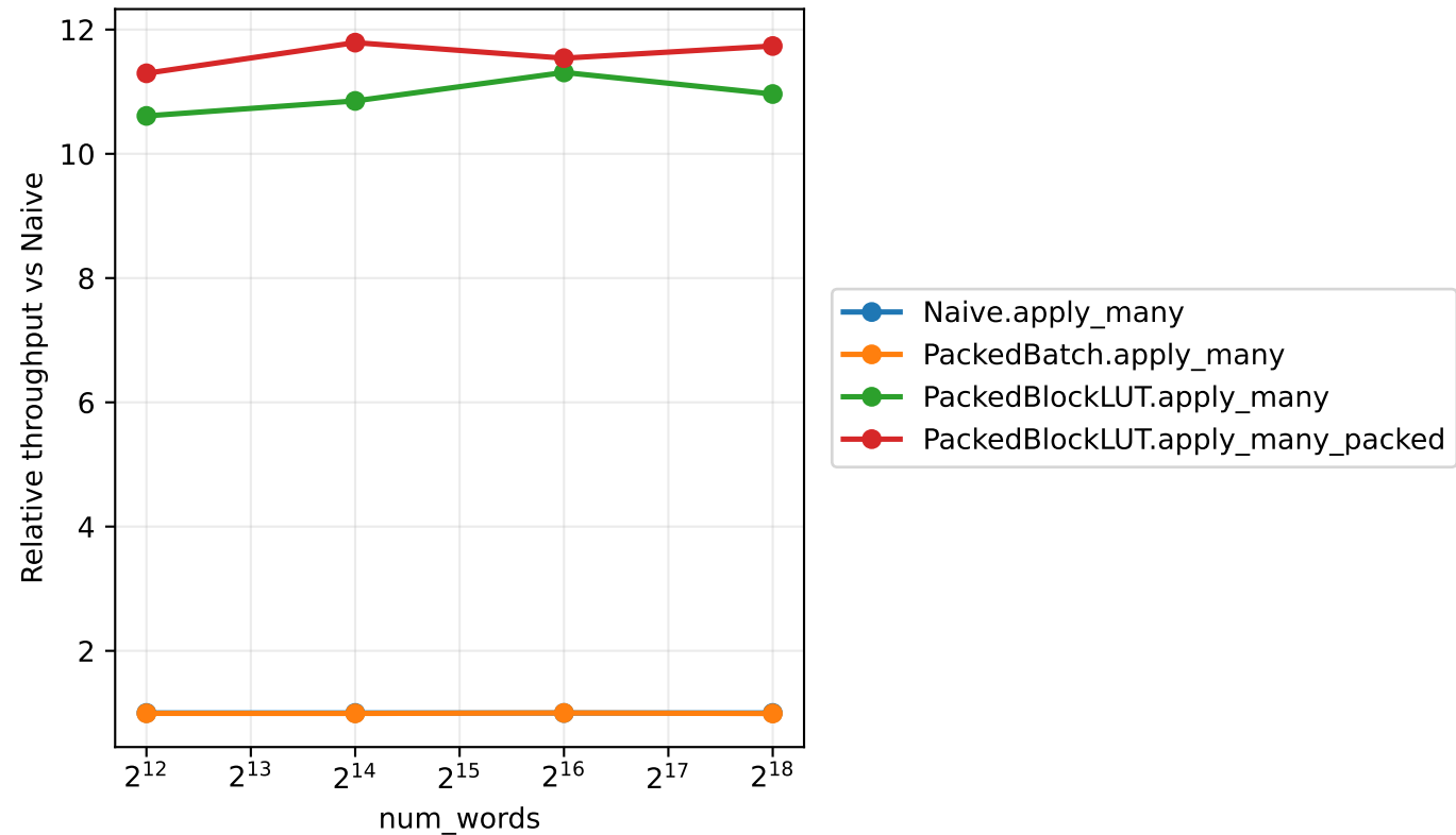
GF(2) component-loop benchmark
