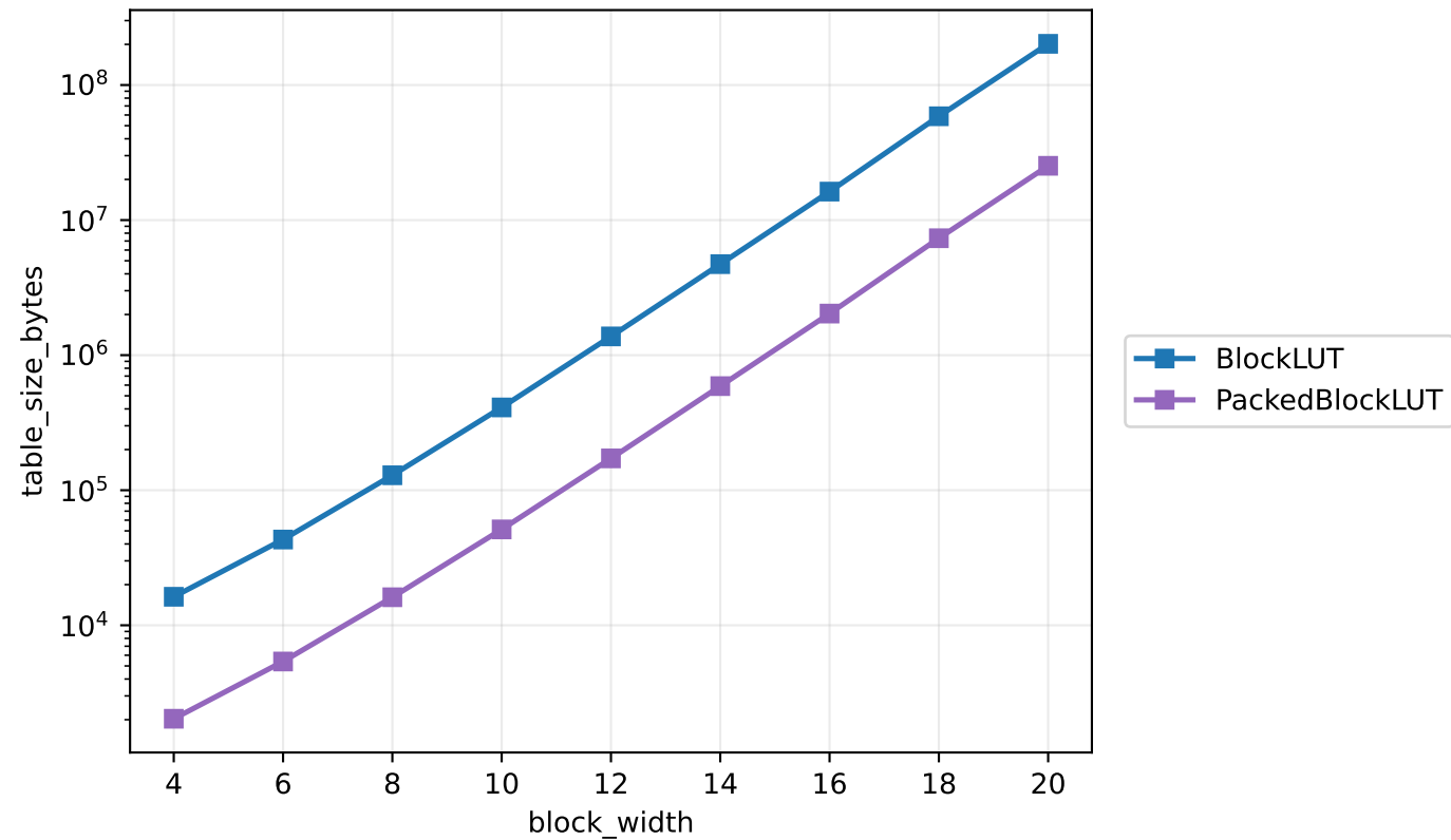
GF(2) block-width table size
