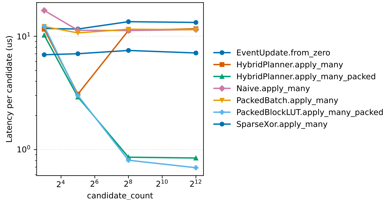
Candidate testing diagnostic
