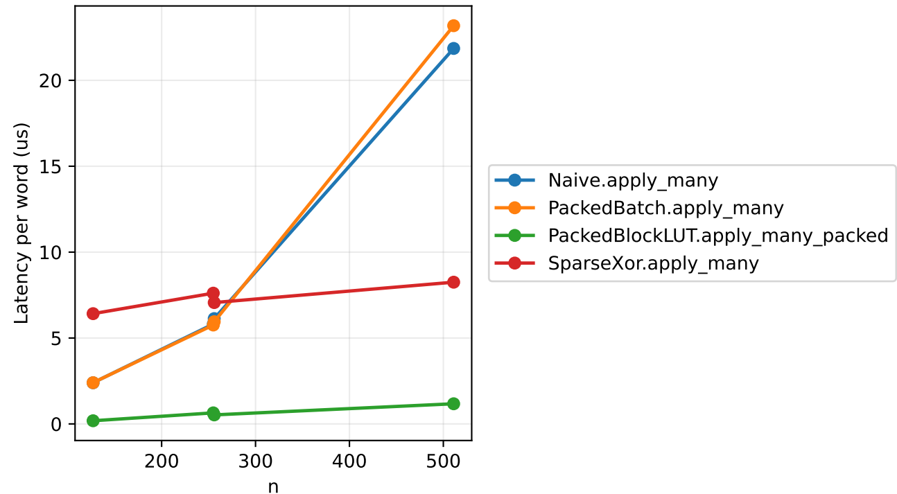
Round 2 code-profile scaling diagnostic
