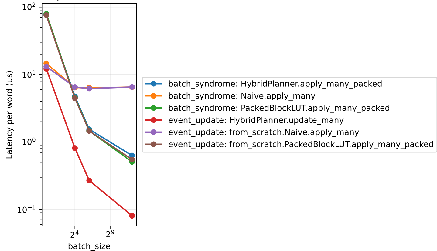
GF(2) planner benchmark
