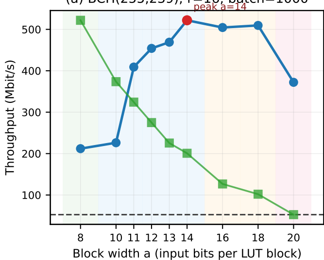
(a) BCH(255,239), r=16 , batch=1000
