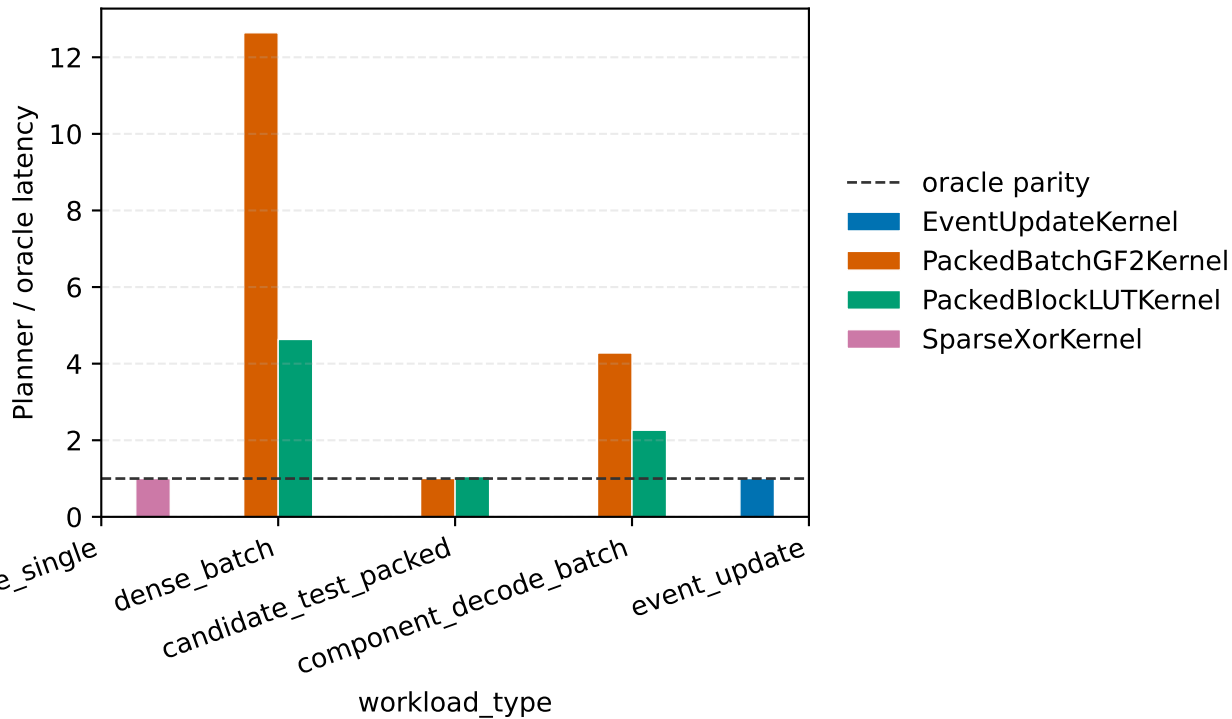
Cache-aware selection diagnostic
