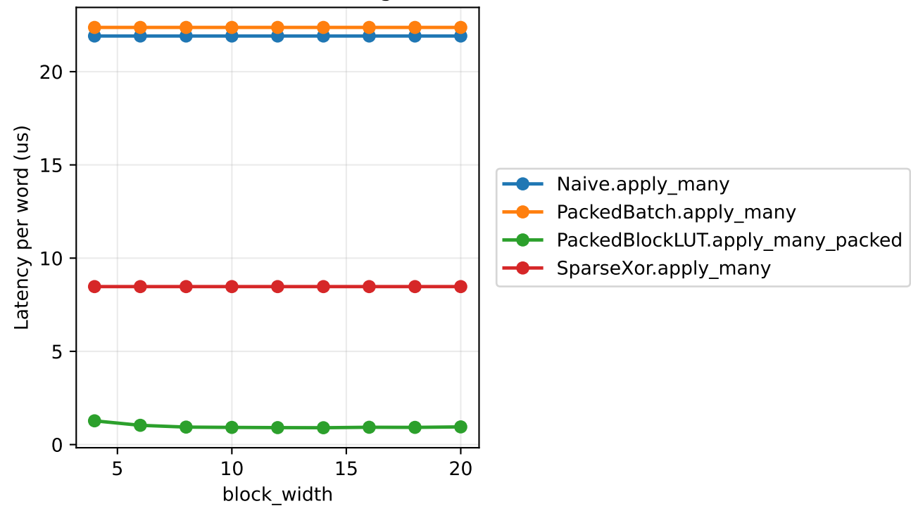
Round 2 cache-aware diagnostic
