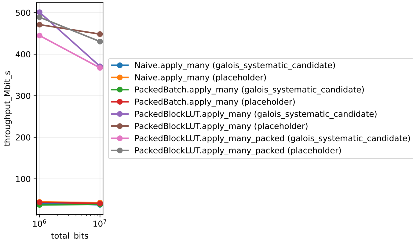
GF(2) component syndrome benchmark
