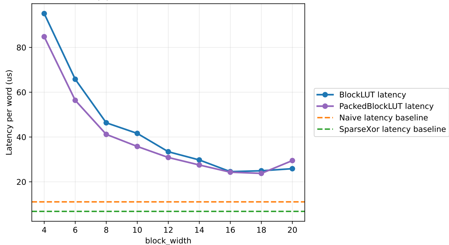
GF(2) block-width micro-benchmark
