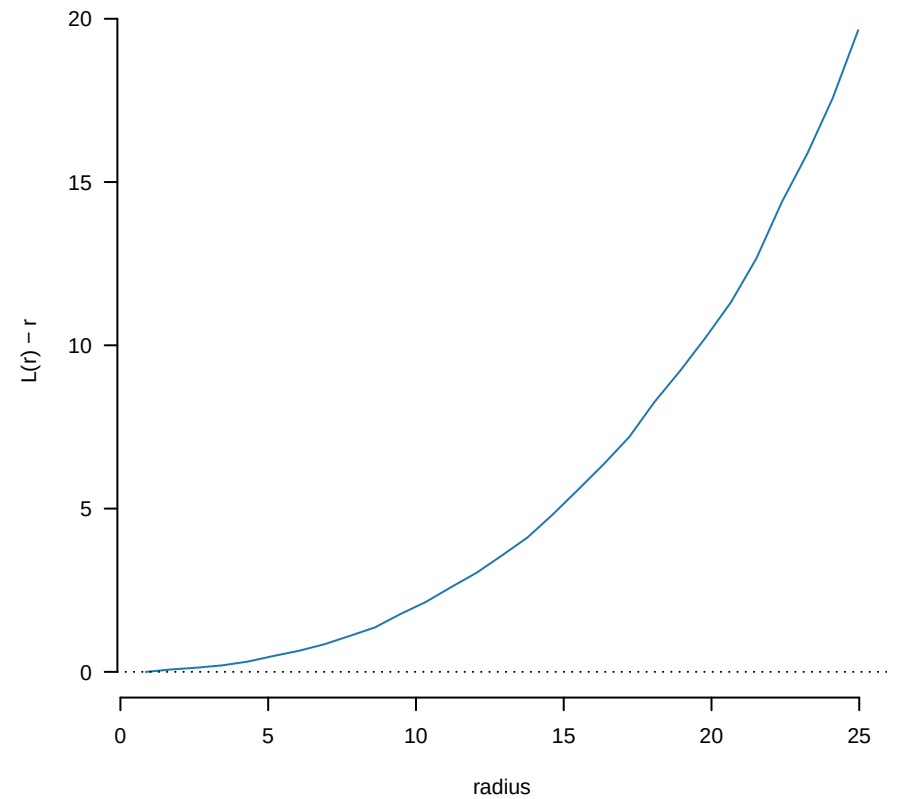
(c) Ripley's L
