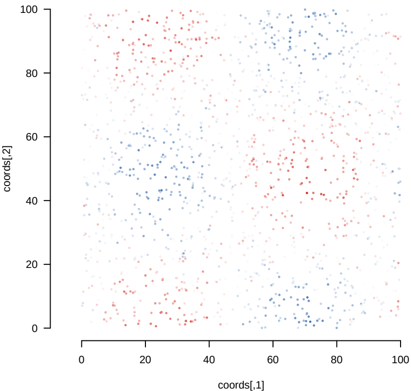
(a) value (Moran I=0.73)
