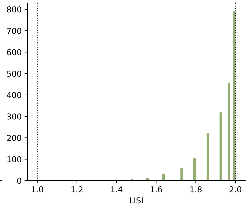
(c) mixing (mean 1.93)
