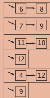
Digraph input format and adjacency-lists representation
