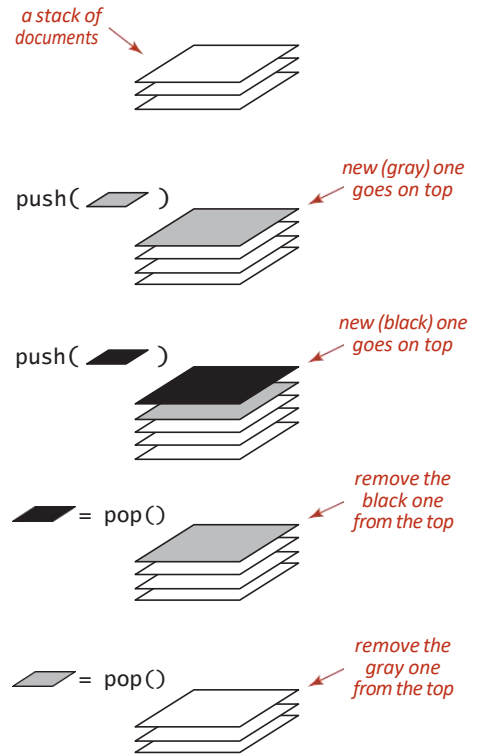
Operations on a pushdown stack
