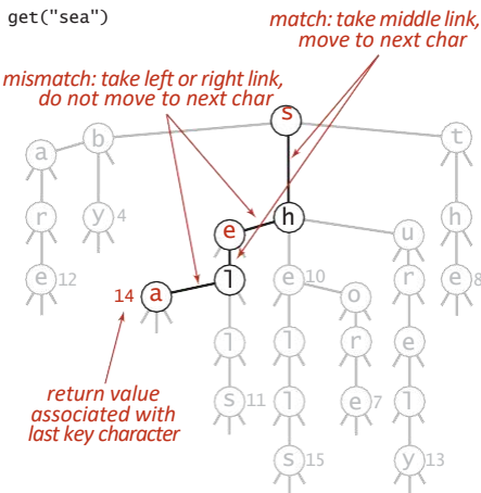
TST search example
