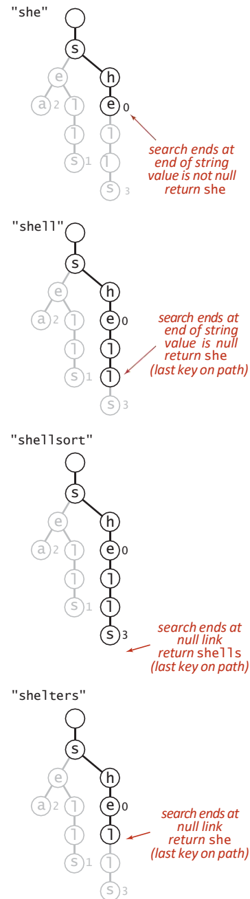
Possibilities for longestPrefixOf()
