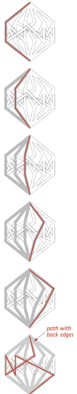
Augmenting paths for bipartite matching
