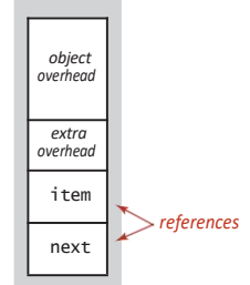
Typical object memory requirements
