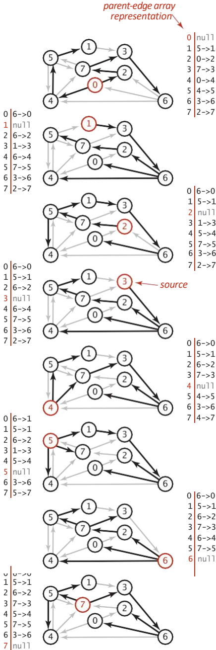
Shortest-paths trees
