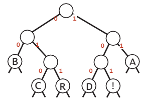
trie representation
