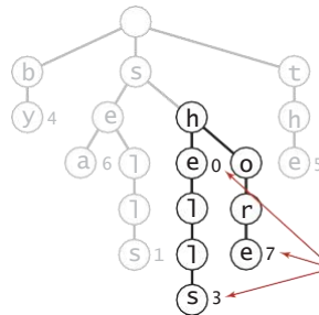
Prefix match in a trie
