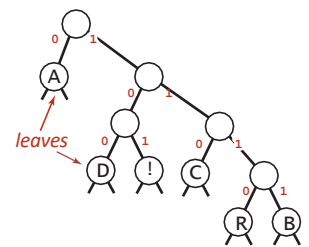
trie representation
