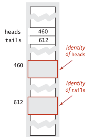
Object representation
