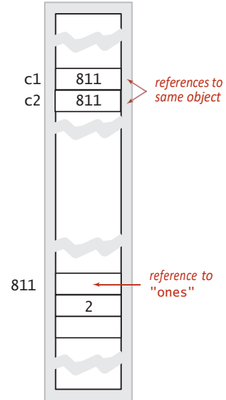
Aliasing
