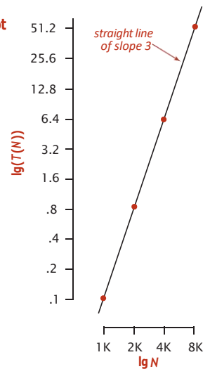
log-log plot
