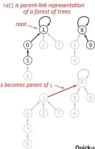
Quick-union overview
