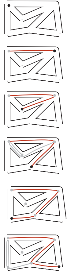
Tremaux exploration
