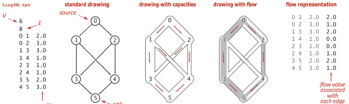
Anatomy of a network-flow problem
