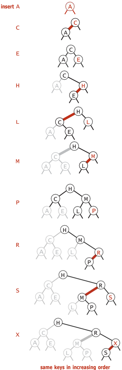
Red-black BST construction traces
