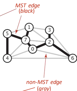
An edge-weighted graph and its MST
