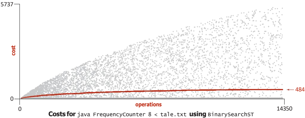
Costs for java FrequencyCounter 8 < tale.txt using BinarySearchST
