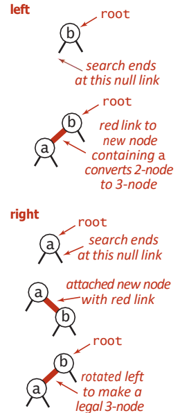
Insert into a single 2-node (two cases)
