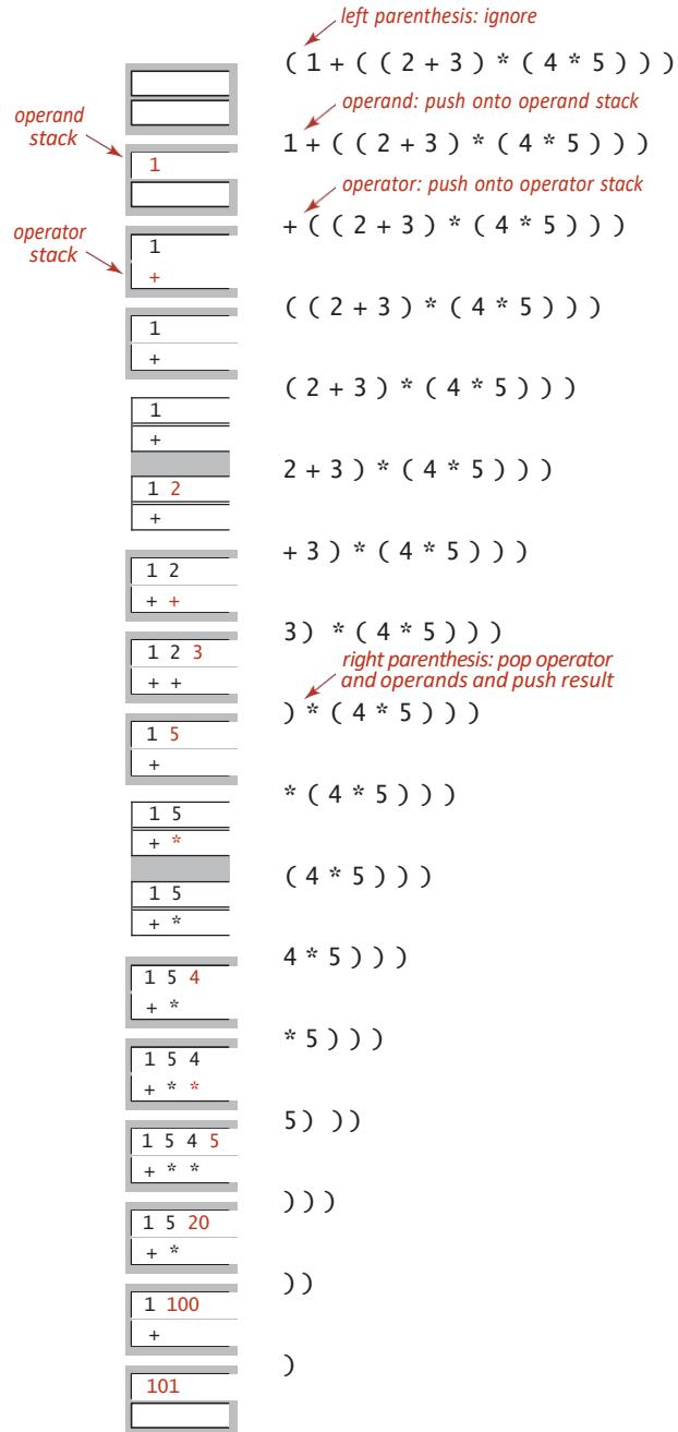
Trace of Dijkstra's two-stack arithmetic expression-evaluation algorithm
