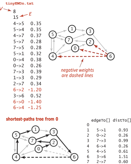
An edge-weighted digraph with negative weights
