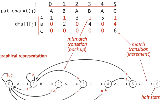
DFA corresponding to the string A B A B A C
