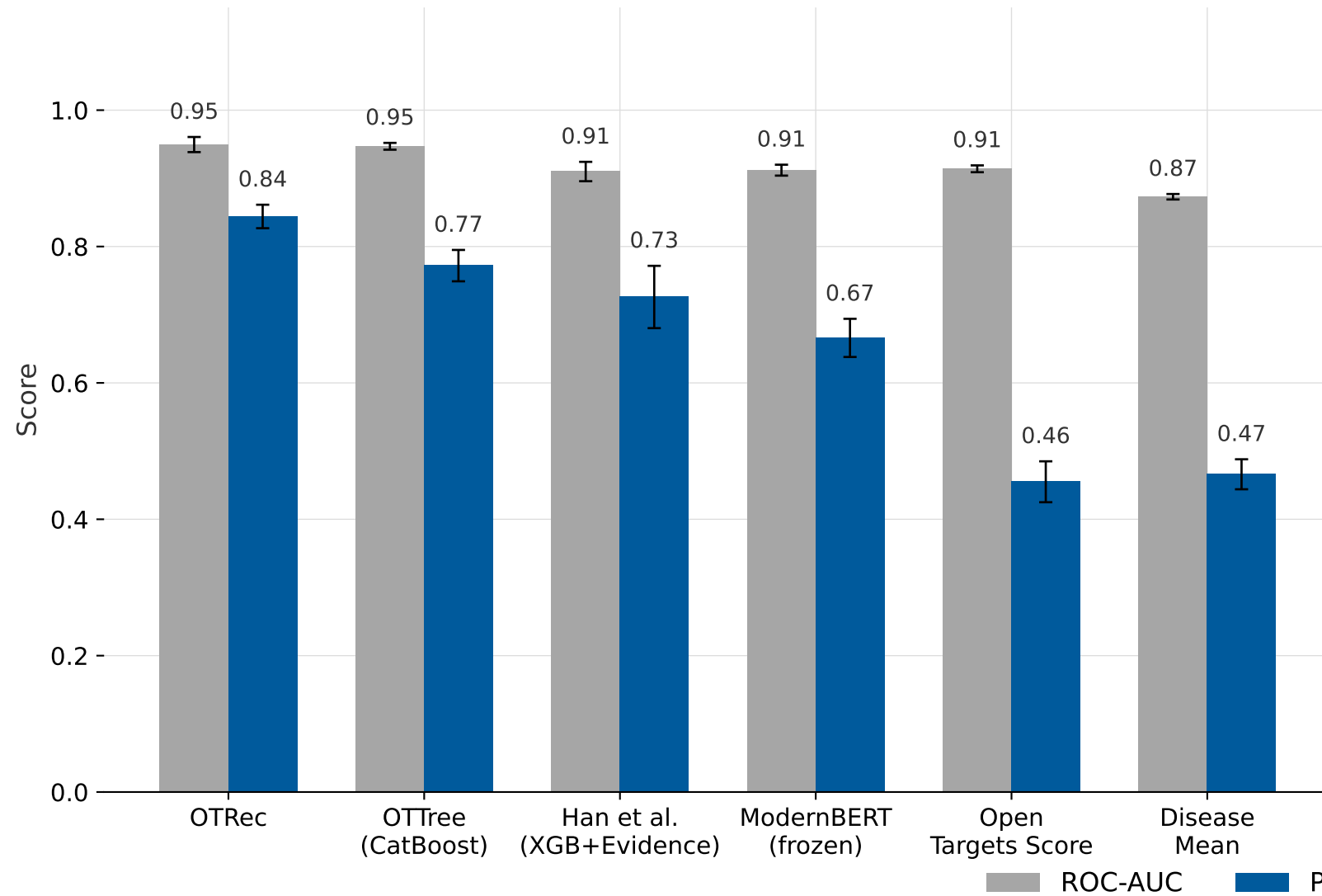
B. Target-Disjoint Cross-Validation (5x5-fold)
