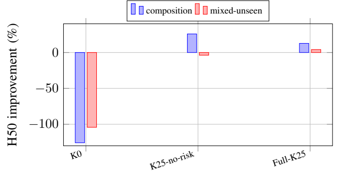
Fig. 2. Seed17 long-horizon mechanism. Context reverses catastrophic K0 drift; depth risk trades peak gain for an all-positive frozen gate.
