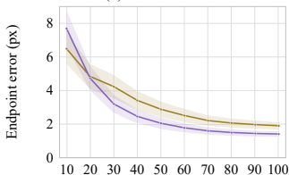
(f) J4 / J5 - Hardware
