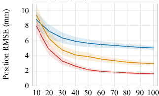
(c) Goal distance - Sim
