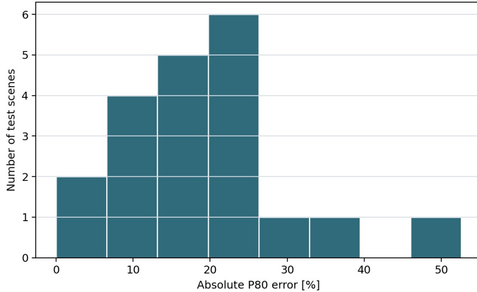
Figure 3. Held-out test distribution of absolute P80 error for the selected EdgeConv post-split setting.
