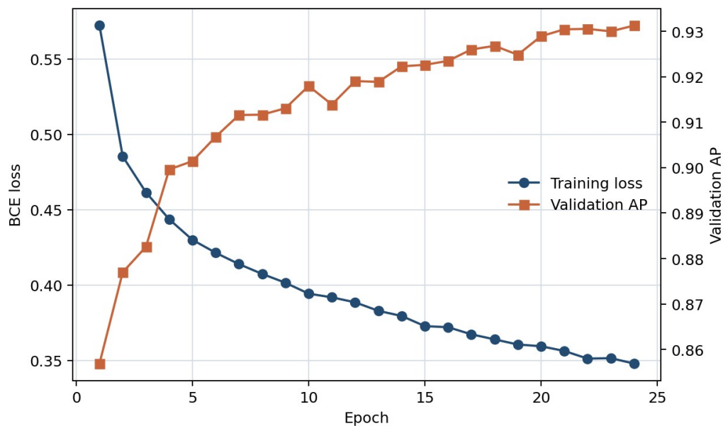
Figure 5. Training loss and validation average precision for the 24-epoch EdgeConv run.
