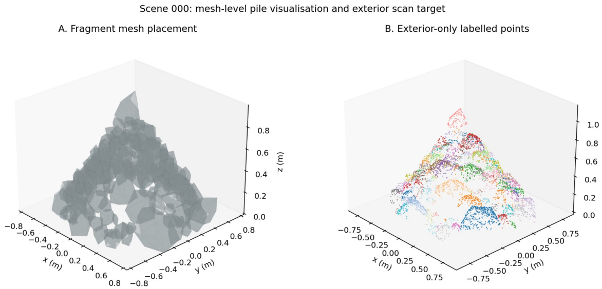
Figure 3. Scene 000 mesh-level pile visualisation and exterior-only labelled point-cloud target.
