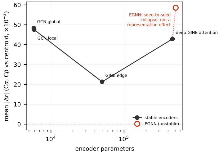
b Representation effect vs capacity
