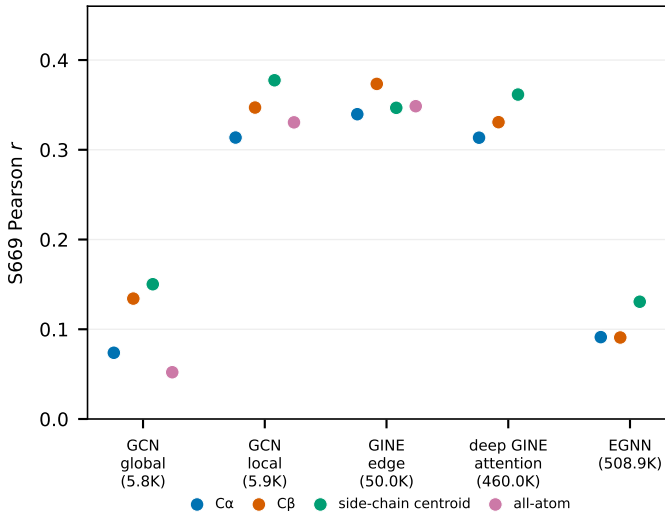
a Model performance by graph definition
