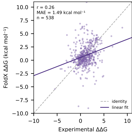
c FoldX energy signal
