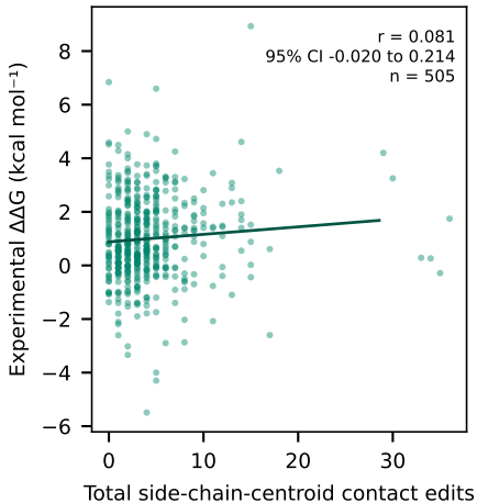
a Unaggregated edit counts
