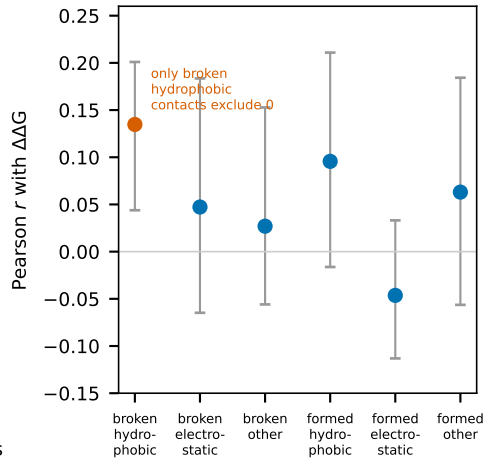
b Contact edits by type
