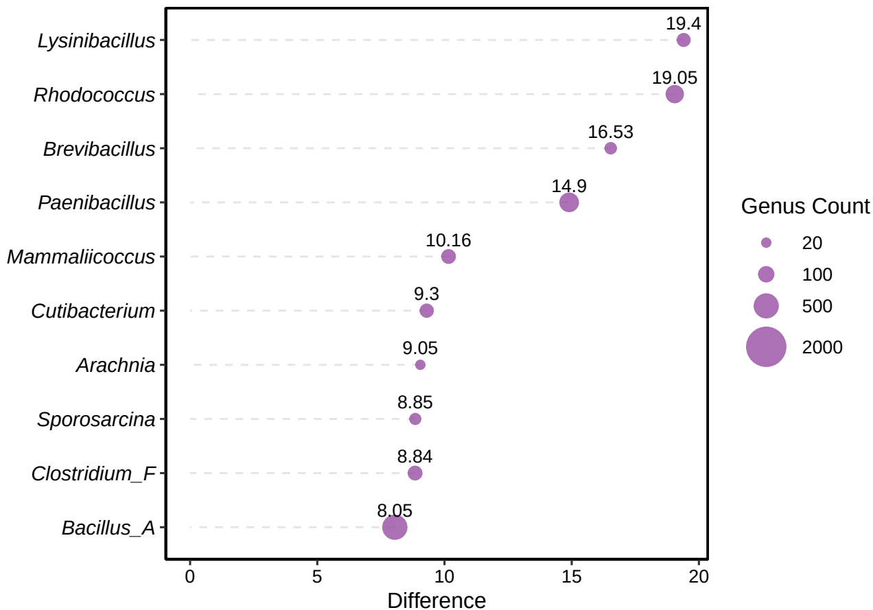
Top 10: Excess Receptors (Avg PBP2 > 1)
