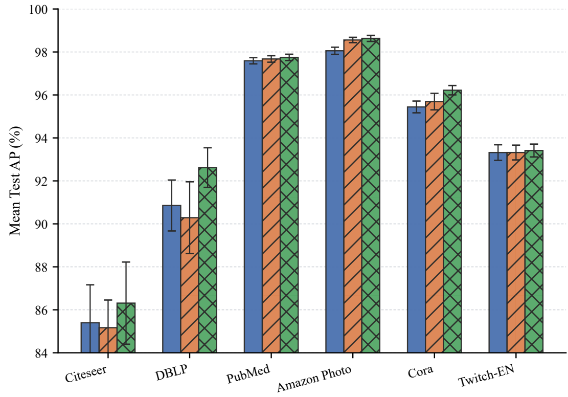
(b) Test AP
