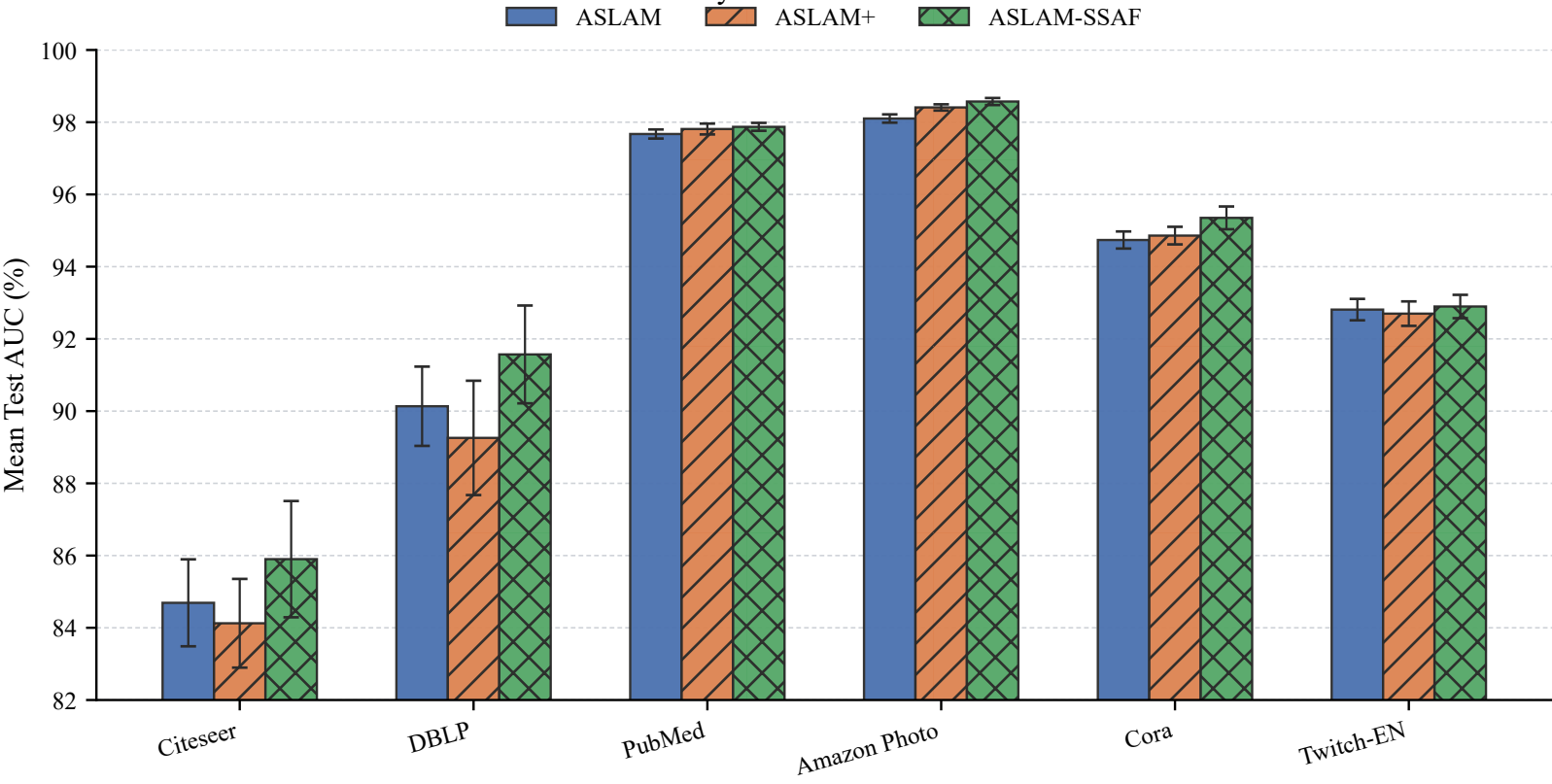
Ablation Study of ASLAM-SSAF: Test AUC
