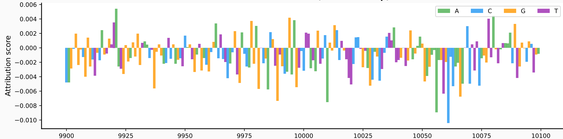
Base-level Attribution (9900-10100bp)
