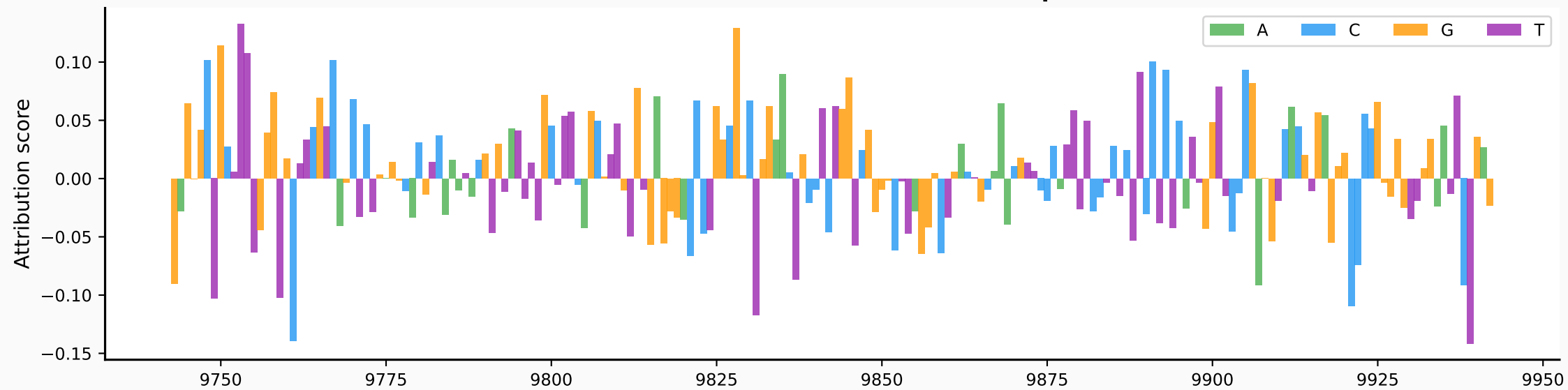
Base-level Attribution (9743-9943bp)
