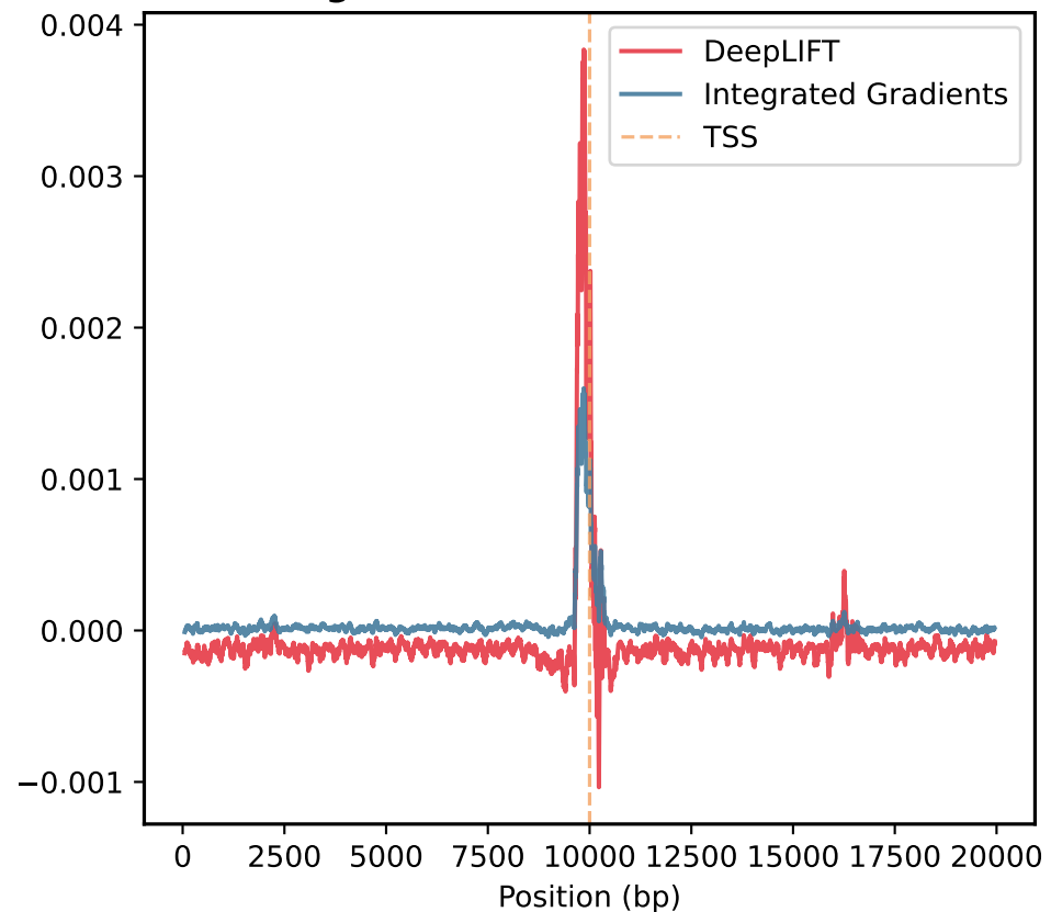
Method Agreement: Global Attribution Profile
