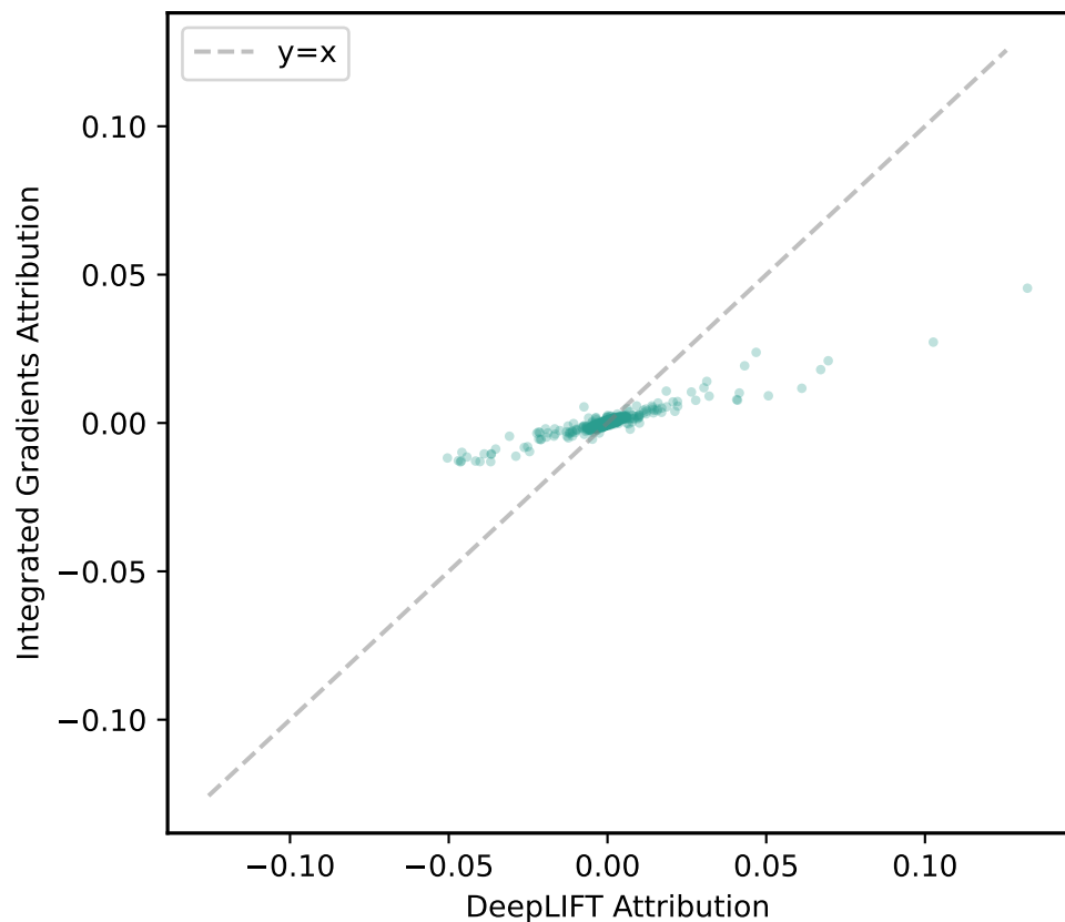
Per-base Attribution Correlation ( r = 0.9442 )
