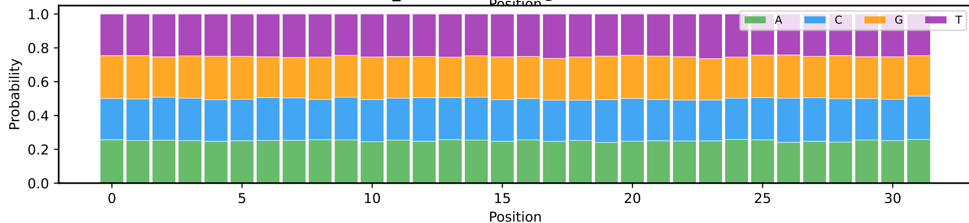
Conv conv_c (k=32): Average Filter Motif (n=5)
