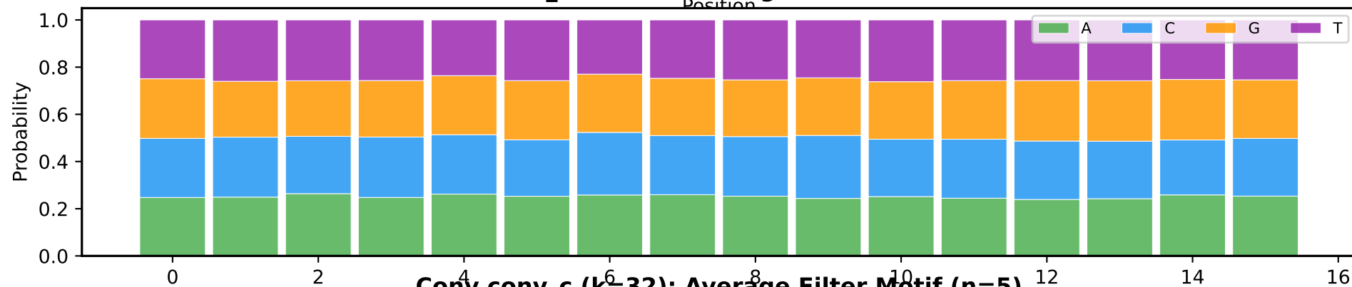
Conv conv_c (k=32): Average Filter Motif (n=5)
