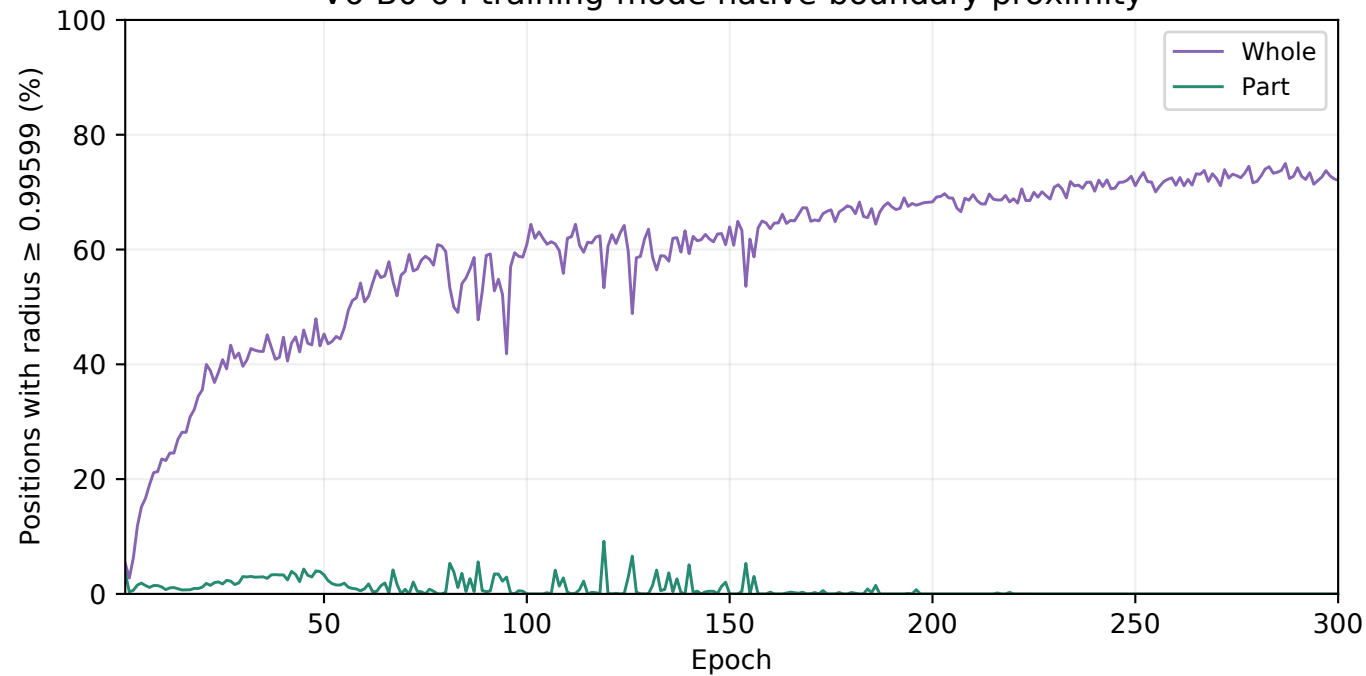
V6-B0-64 training-mode native-boundary proximity
