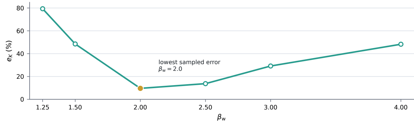
Fibrous proxy wall-coefficient sensitivity
